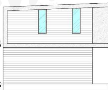
ELEVATION-B
