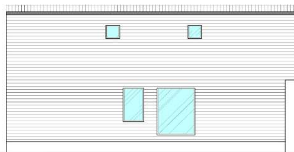
ELEVATION-C
