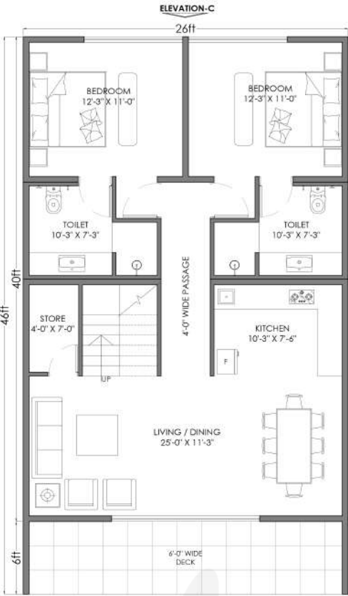
CABANA 'A' - 3BHK GROUND FLOOR PLAN COVERED AREA = 1196 Sq.Ft BUILT UP AREA = 1664 Sq.Ft
