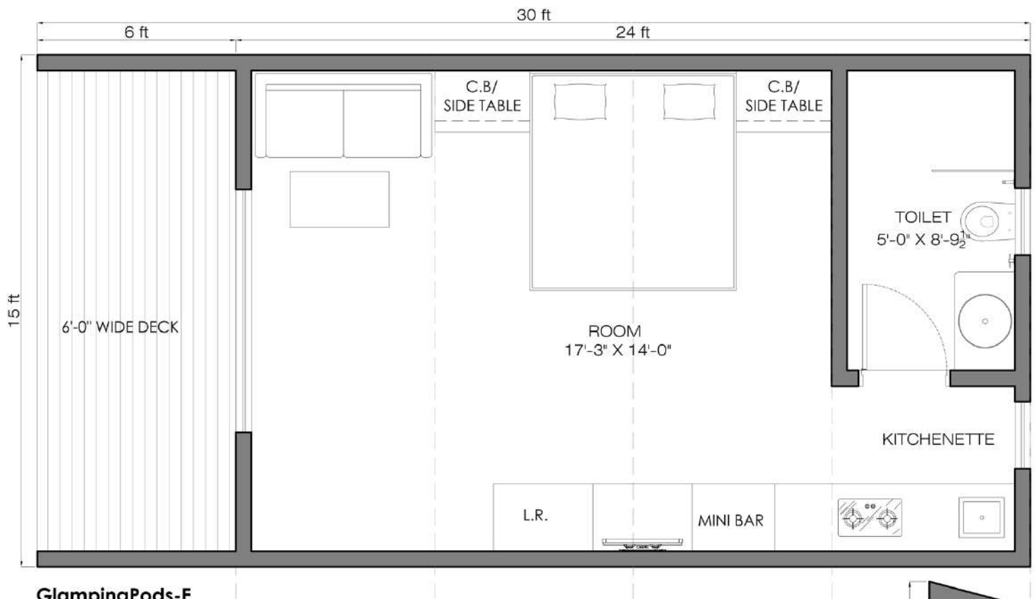
GlampingPods-E COVERED AREA = 450 Sq.Ft
