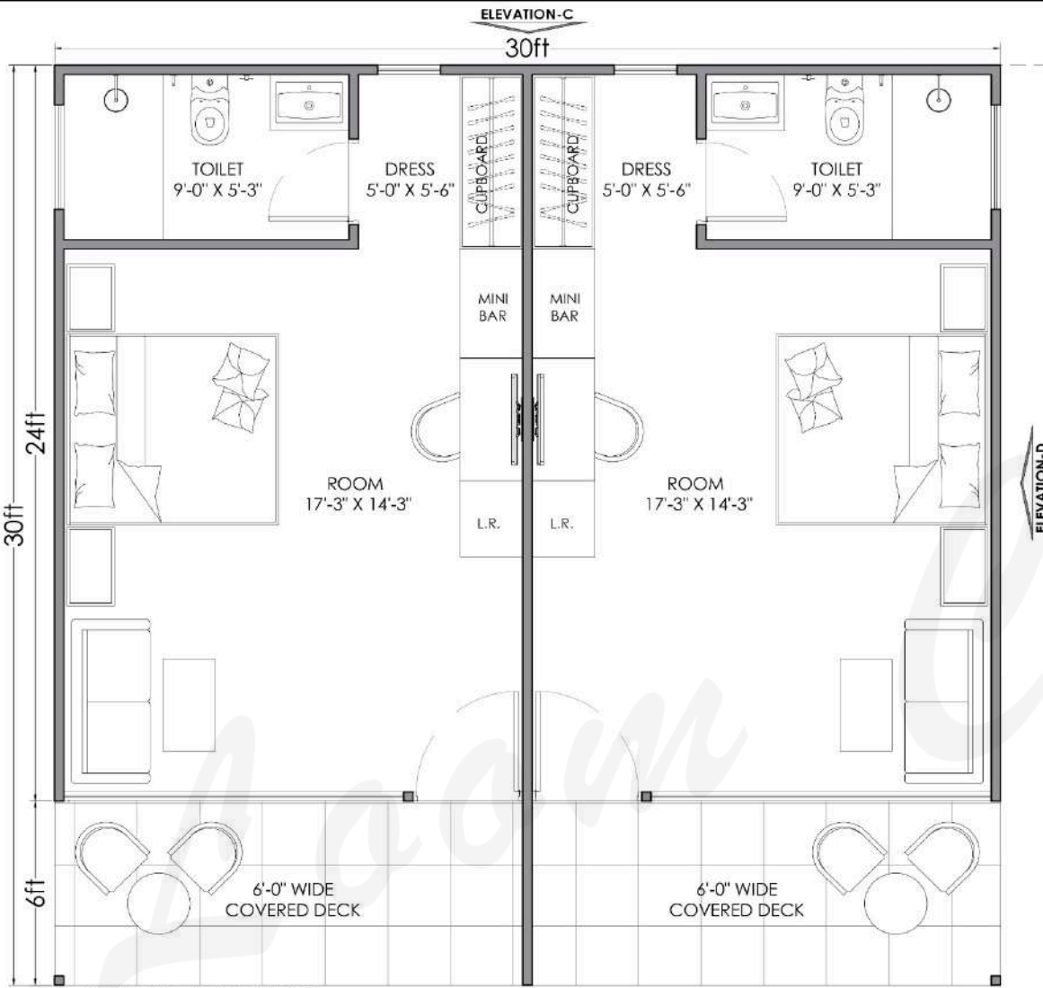
TWIN ROOM COTTAGE GROUND FLOOR PLAN COVERED AREA = 900 Sq.Ft
