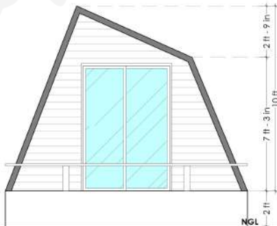
ELEVATION-B
