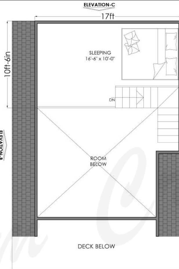
ELEVATION-A CABANA A FRAME SINGLE ROOM-LOFT MEZZANINE FLOOR
