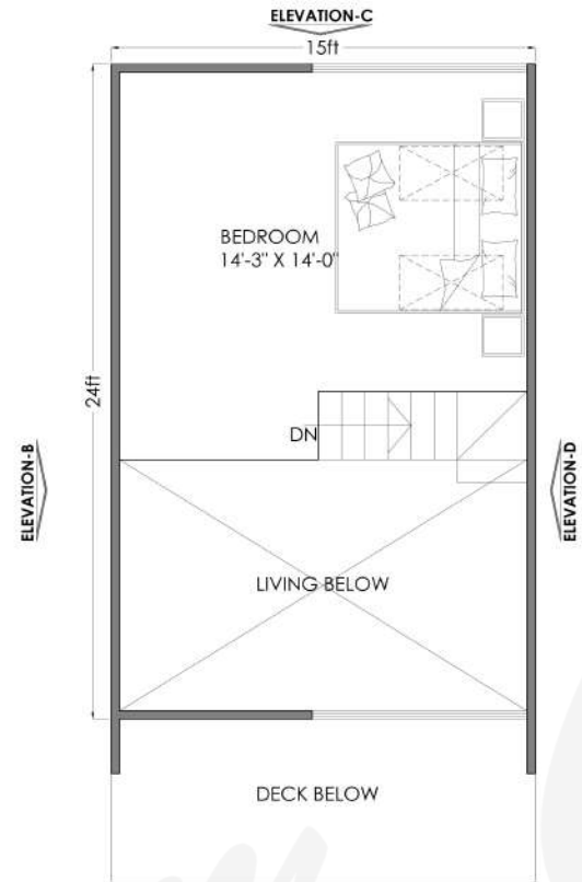
MODROOM-XL LOFT MEZZANINE FLOOR PLAN COVERED AREA = 260 Sq.Ft DOUBLE HEIGHT AREA = 130 Sq.Ft
