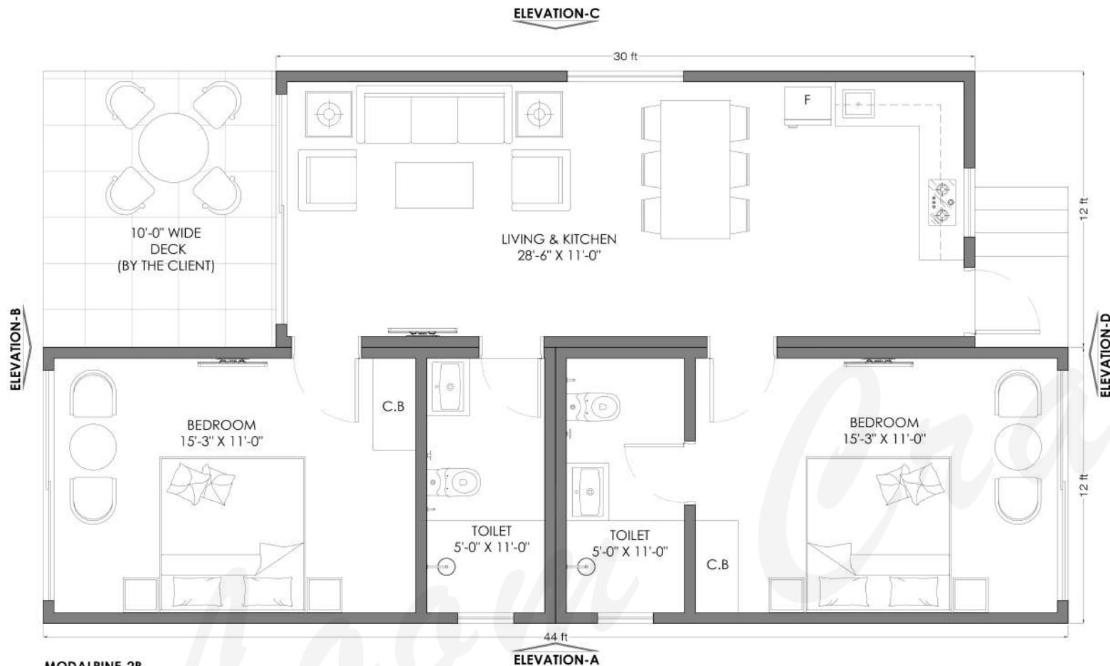
MODALPINE-2B FLOOR PLAN COVERED AREA = 888 Sq.Ft
