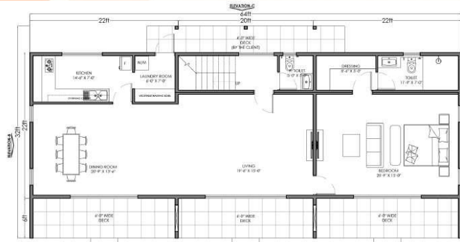
GROUND FLOOR PLAN COVERED AREA = 1408 Sq.Ft COVERED DECK AREA = 384 Sq.Ft TOTAL BUILT UP AREA = 3476 Sq.Ft
